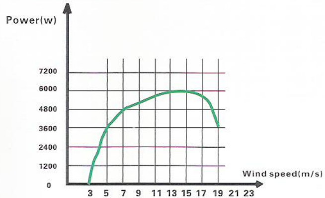
500W wind speed and power diogram of curves
