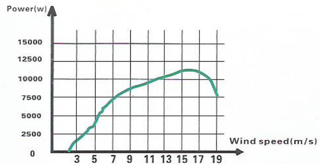
2000W wind speed and power diogram of curves
